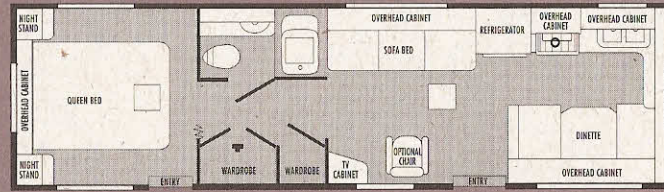
Available with Options A, B, or H 30FK
