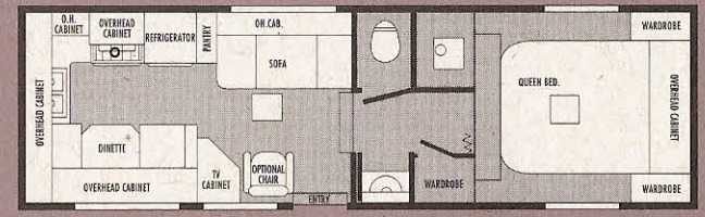
Available with Options D or H 27RK
