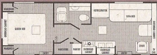
Available with Option A 25FS
