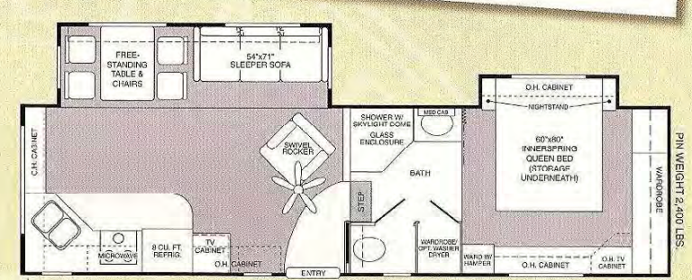
FIFTH WHEEL F-304 SR LENGTH: 31' 11" • WIDTH: 8"
