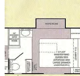
FIFTH WHEEL F-297 SR LENGTH: 31' 10" • WIDTH: 8"
