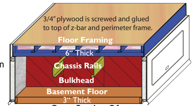
Cross Section Of Main Floor, Frame, Chassis & Basement Floor
