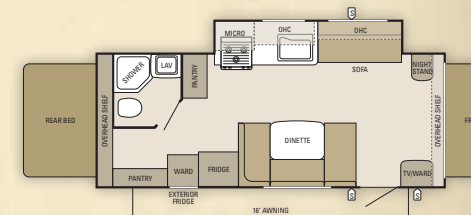
Travel Star EXP 227CKS
