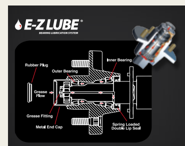
E-Z lube axles allow you to lubricate your wheel bearings quickly and easily without disassembly
