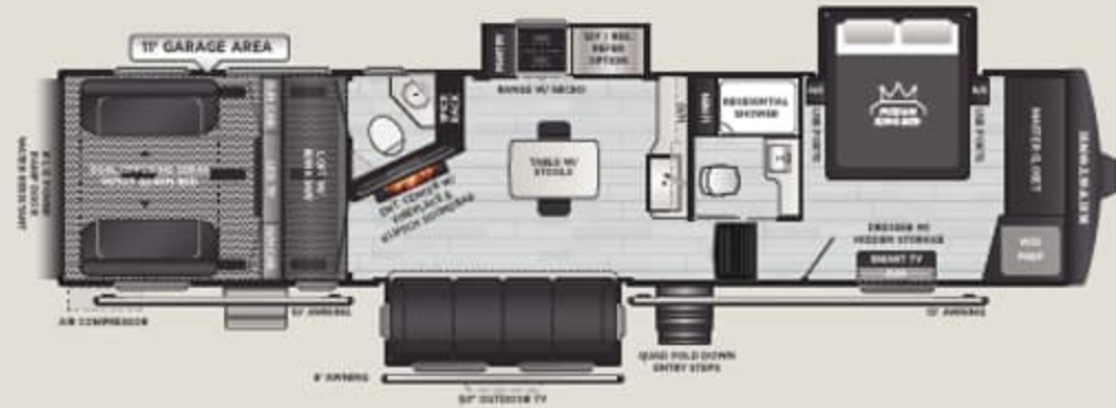
373 | WEIGHT 16325 | LENGTH 39' 6"
