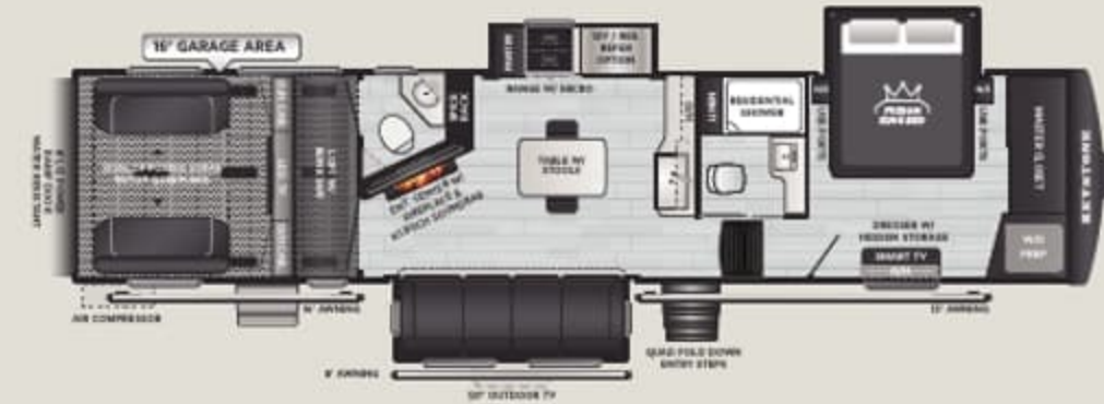
419 | WEIGHT 16935 | LENGTH 44' 6"
