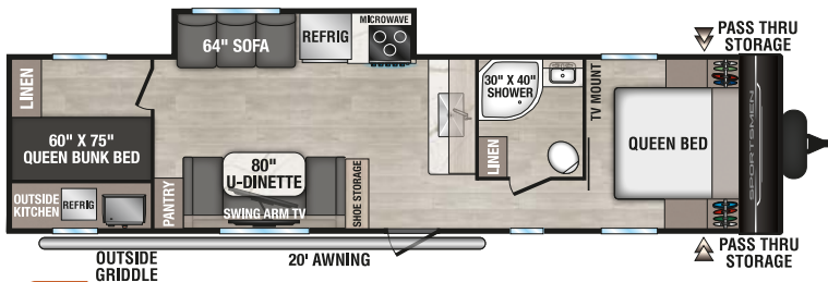
321BHK UVW - 7,050 | Exterior Length - 36' 7" | Sleeps - 9
