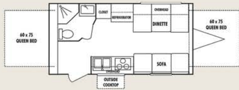
20C •UVW 3352 • Length 20'8"
