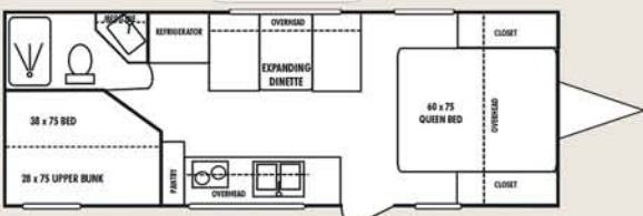
CL230 •UVW 3705 • Length 27'0"
