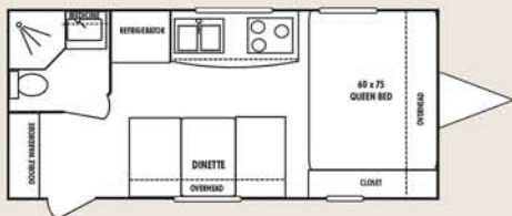
CL164 •UVW 2886 • Length 20'5"
