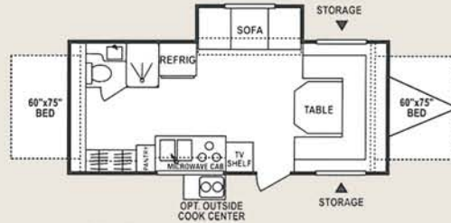
23CMS •UVW 4166 • Length 24'7"
