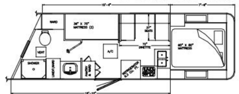
15' living quarters package
