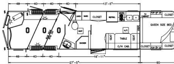
13' living quarters package
