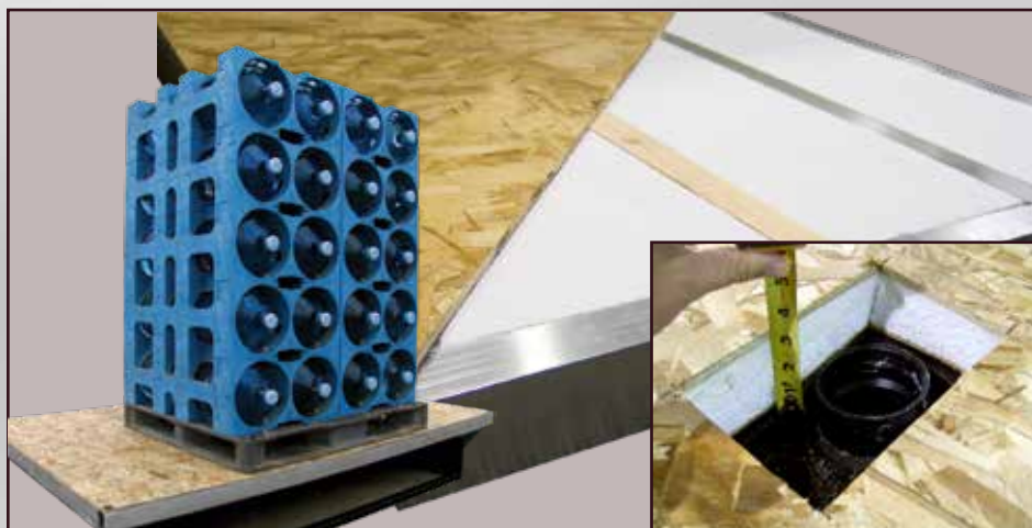
R38 Laminated floor system - Industries lightest and strongest. The 3" thick laminated floor provides maximum strength and insulation.
