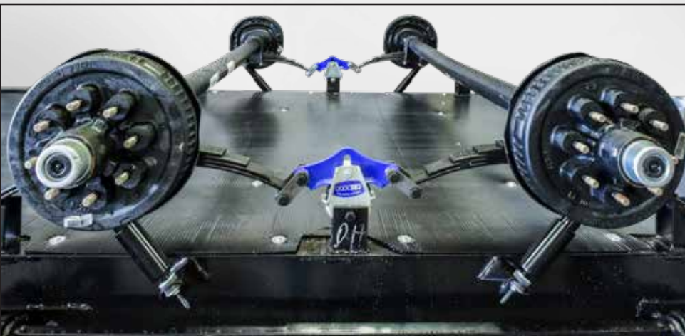
Our industry leading suspension includes four shocks, 7000# Dexter Axles and Mor/Ryde CRE3000 equalizer to provide a smooth ride with less sway and vibrations.
