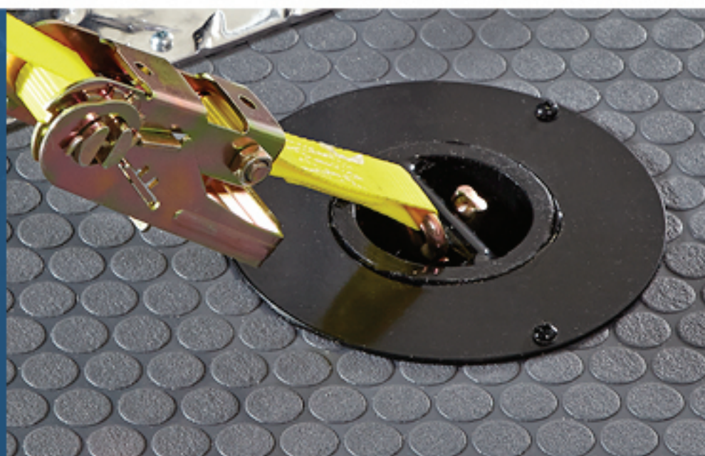
5K Interlock Tie-Down System Industry-leading 5,000 lb. capacity tie-downs for increased safety & security.
