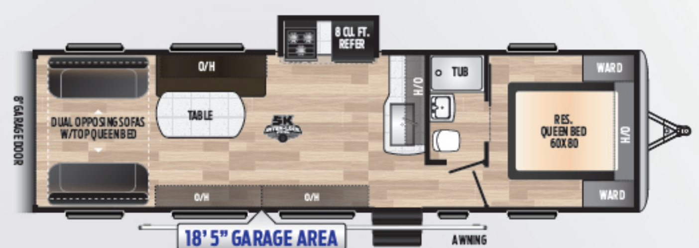
3118 | Open concept, tandem-axle, one slide, 18' 5" garage Weight: 8394 LBS. | Length: 35' 6"
