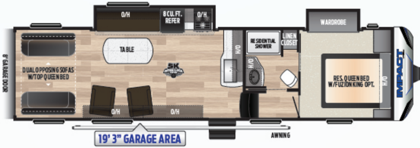
3219 | Open concept, tandem-axle, two slides, 19'3" garage Weight: 10850 LBS. | Length: 35' 8"
