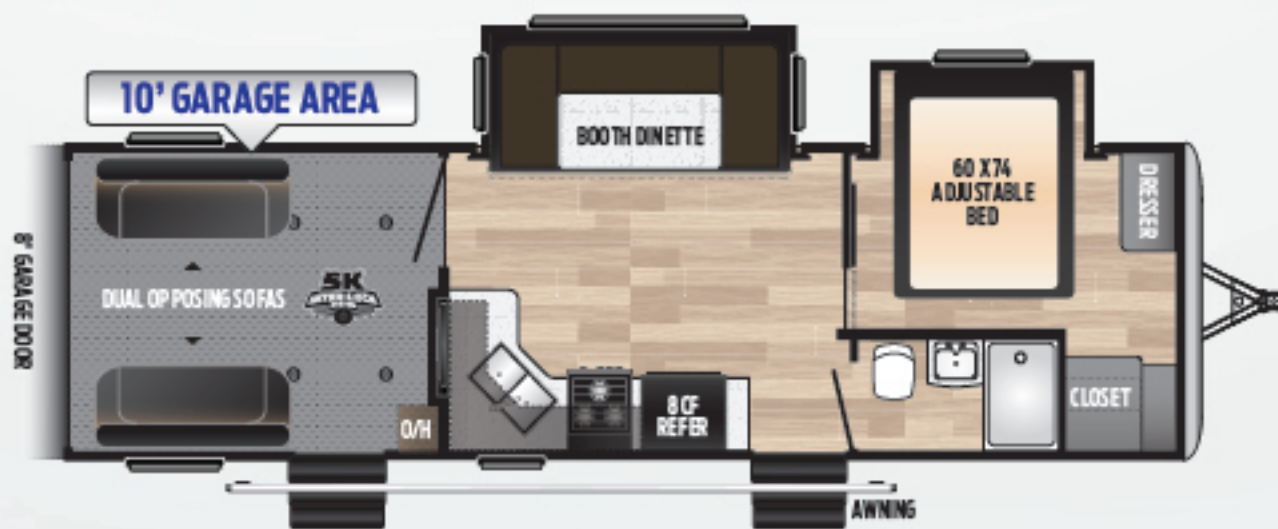
29V | Light weight, tandem-axle, two slides, 10' garage Weight: TBD LBS. | Length: 33' 10"
