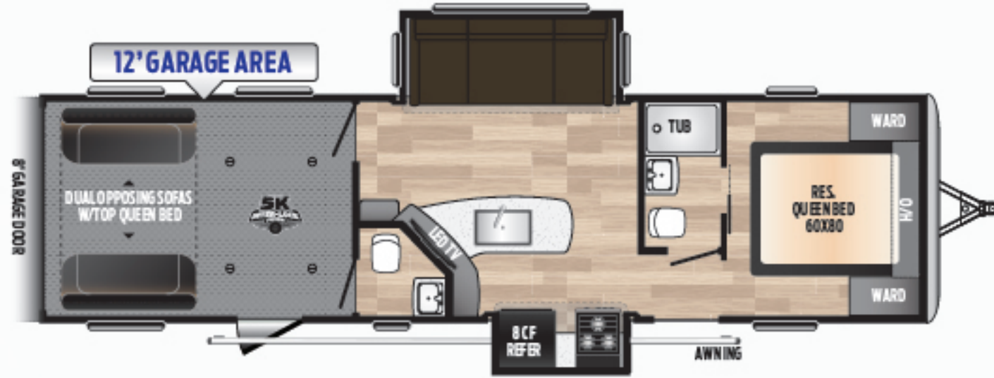
332 | Tandem-axle, 1 1/2 bath, 12' garage Weight: 9648 LBS. | Length: 37' 6"
