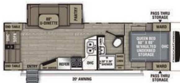
279 RLDS / Exterior Length 31' 10"
