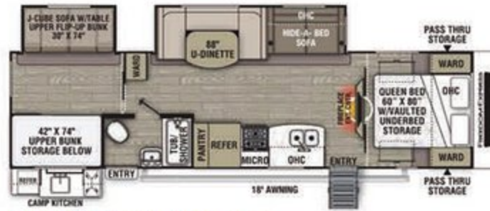
310 BHSLE / Exterior Length 35' 6"
