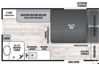
12.0 TD PREMIER UNDER 2,500 LBS.
