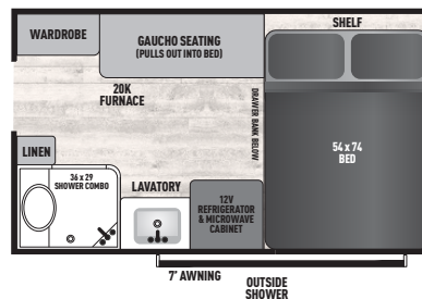
12.0 TD PRO UNDER 2,500 LBS./PULL-OUT KITCHEN
