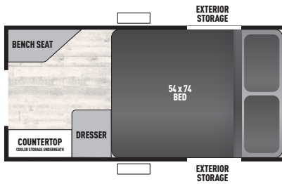
ESCAPE 9.0 TD GARAGE-ABLE!
