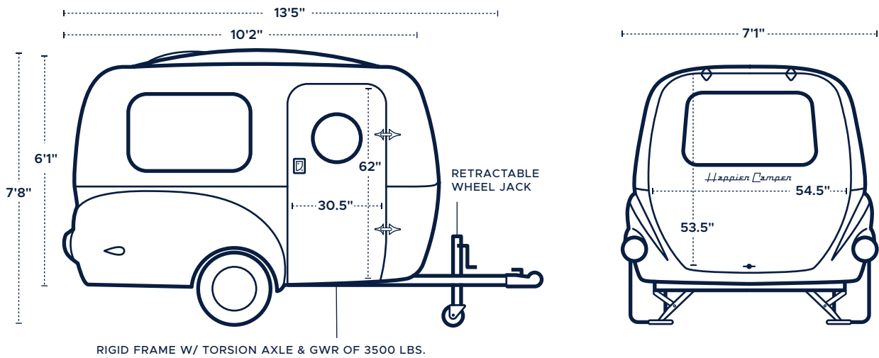
RIGID FRAME W/ TORSION AXLE & GWR OF 3500 LBS.
