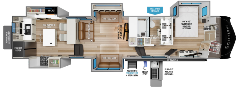
390RK UVW 1 15,000 HITCH 1 2,794 GVWR 19,000 LENGTH 2 42' 5" HEIGHT 3 13' 5" CAPACITY 83 106 53
